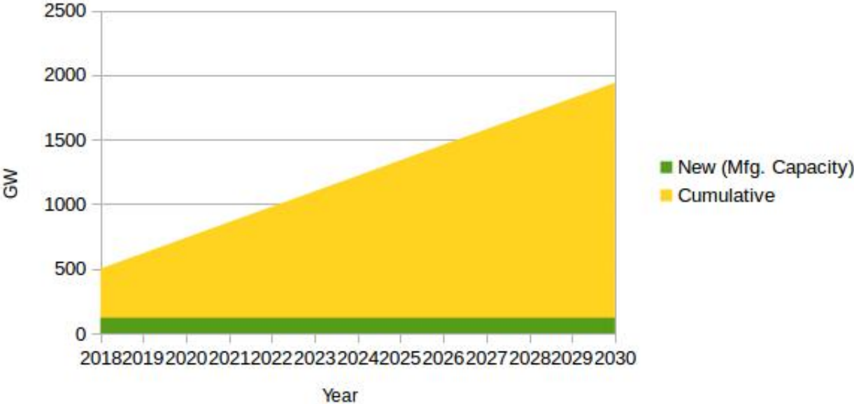
Projected Global Solar PV growth to 2030
